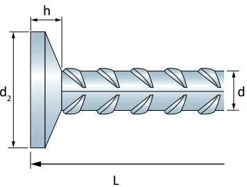
Typ / type 1 (ancoFIX®)
